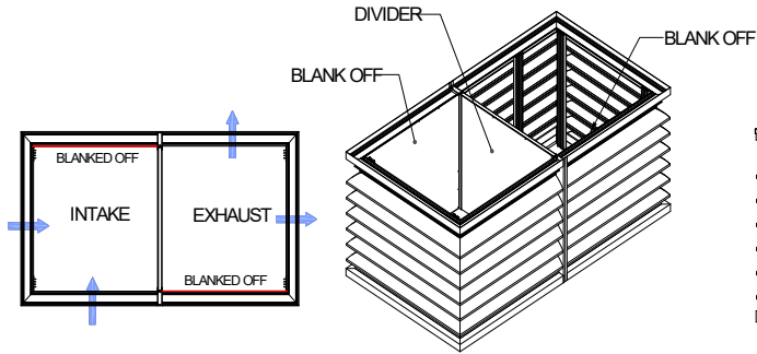
DIVIDER / BAFFLE
