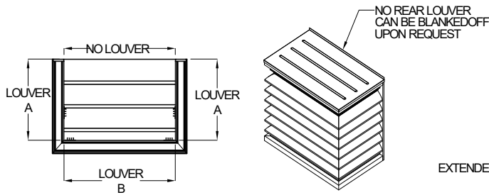
3 SIDED PENTHOUSE
